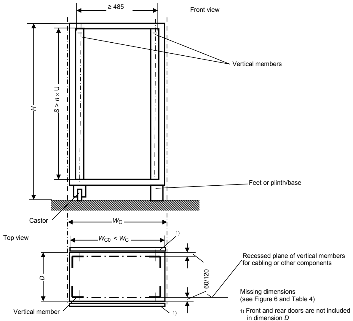
Figure 7 – Dimensions of cabinet type A
