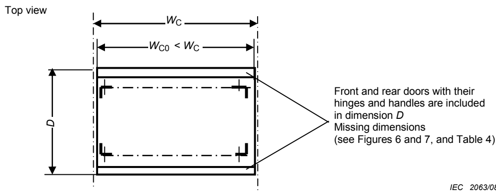
Figure 8 – Dimensions of cabinet type B
